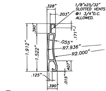
B TYPE 2 SLAT: RLL-3 SLAT EXTRUDED ALUMINUM 6063-T5 ALUMINUM ALLOY SCALE: 1/2" = 1"
