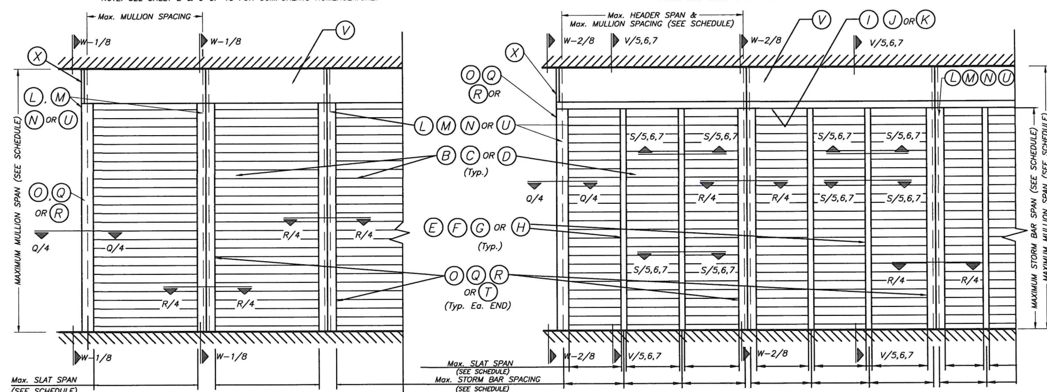
TYPICAL CONSECUTIVE SINGLE UNIT ELEVATION (NO STORM BARS REQUIRED) NOTE: SEE SHEET 2 & 3 OF 13 FOR COMPONENTS NOMENCLATURE. TYPICAL CONSECUTIVE MULTIPLE UNIT ELEVATION (STORM BARS REQUIRED) NOTE: SEE SHEET 2 & 3 OF 13 FOR COMPONENTS NOMENCLATURE.
