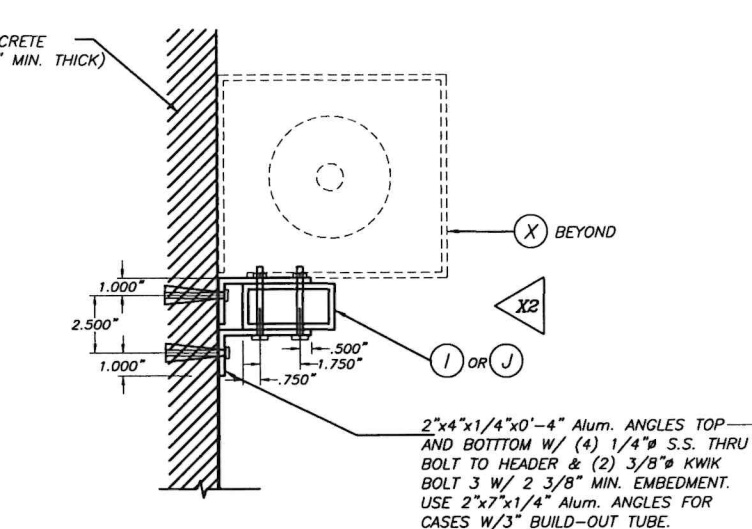
ALTERNATIVE 3 WALL MOUNTING : SECTION W-W(3) SCALE : 1/8" = 1"
