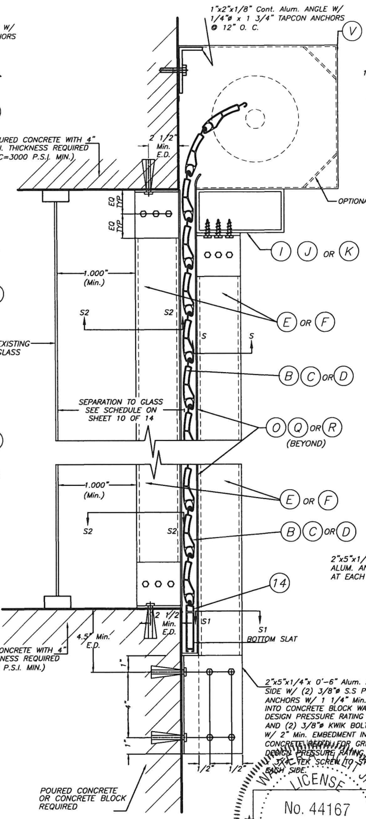
WALL MOUNTING: SECTION V-V(1) INSTALLATION W/ FIXED STORM BARS W/CONCRETE ANCHORS SCALE : N.T.S.
