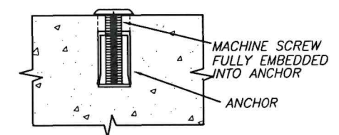
DETAIL A SCALE : 1/2" = 1" * 1/4" Ø-20 OR 3/8" Ø-16 S.S. MACHINE SCREWS USED JOINTLY W/ 1/4" Ø x 7/8" OR 3/8" Ø x 1 1/4" CALK-IN ANCHORS RESPECTIVELY SHALL BE LEFT TOGETHER W/ ANCHORS AT THE TIME STORM BARS ARE REMOVED. (SEE DET. A).
