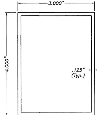
M TYPE 2 MULLION: 4" EXTRUDED MULLION 6063-T5 ALUMINUM ALLOY SCALE: 1/2" = 1"
