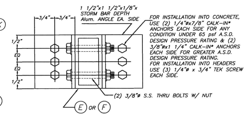
SECTION S - S (FOR REMOVABLE STORM BAR) SCALE : N.T.S.
