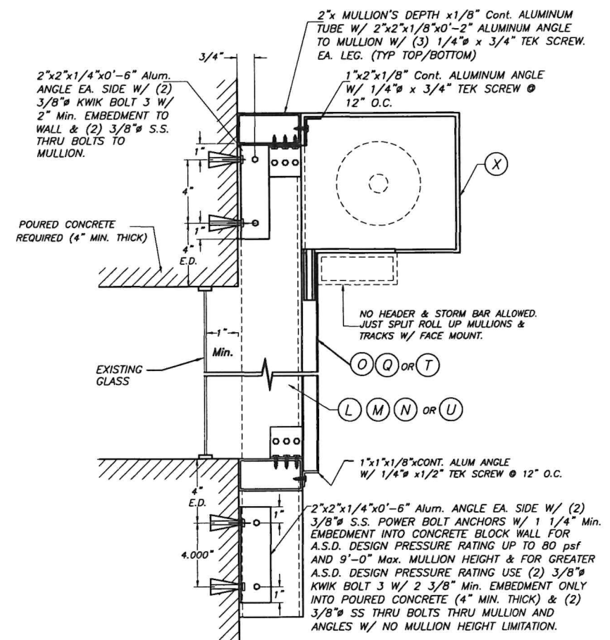
WALL MOUNTING : MULLION CONNECTION AT TOP & BOTTOM : SECTION W-W (1) SCALE : 1/8" = 1"
