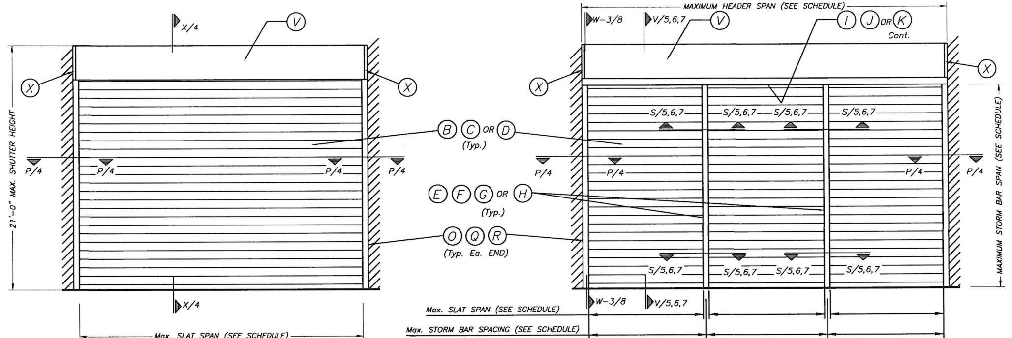
TYPICAL SINGLE UNIT ELEVATION (NO STORM BARS REQUIRED) NOTE: SEE SHEET 2 & 3 OF 13 FOR COMPONENTS NOMENCLATURE. TYPICAL MULTIPLE UNIT ELEVATION (STORM BARS REQUIRED) NOTE: SEE SHEET 2 & 3 OF 13 FOR COMPONENTS NOMENCLATURE.
