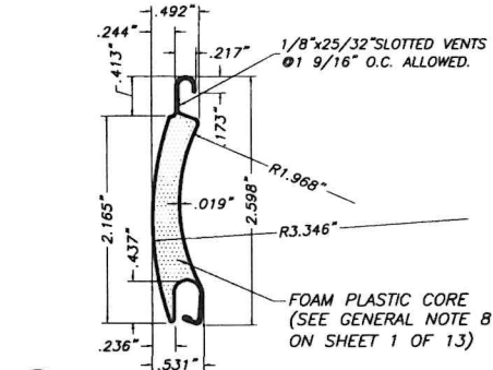
C TYPE 3 SLAT: A-200-H SLAT 55mm (t = .019") HIGH DENSITY FOAM PLASTIC CORE SHEET METAL ALUMINUM SLAT 3005-H48 ALUMINUM ALLOY SCALE: 1/2" = 1"
